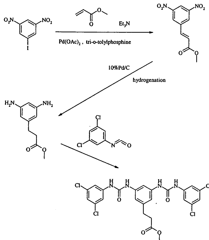
Scheme III-A
